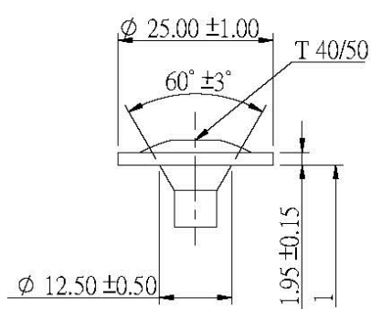
Washer Head
