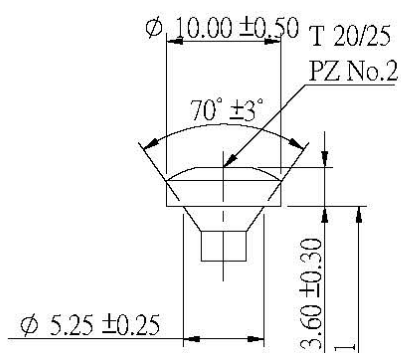
Pan Head
