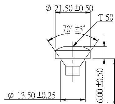
Pan Head
