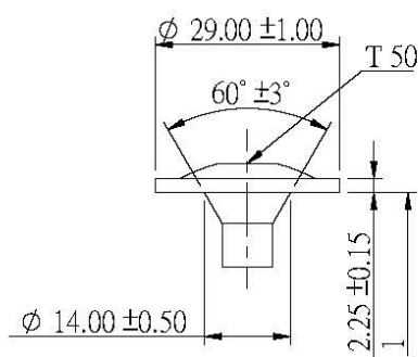
Washer Head
